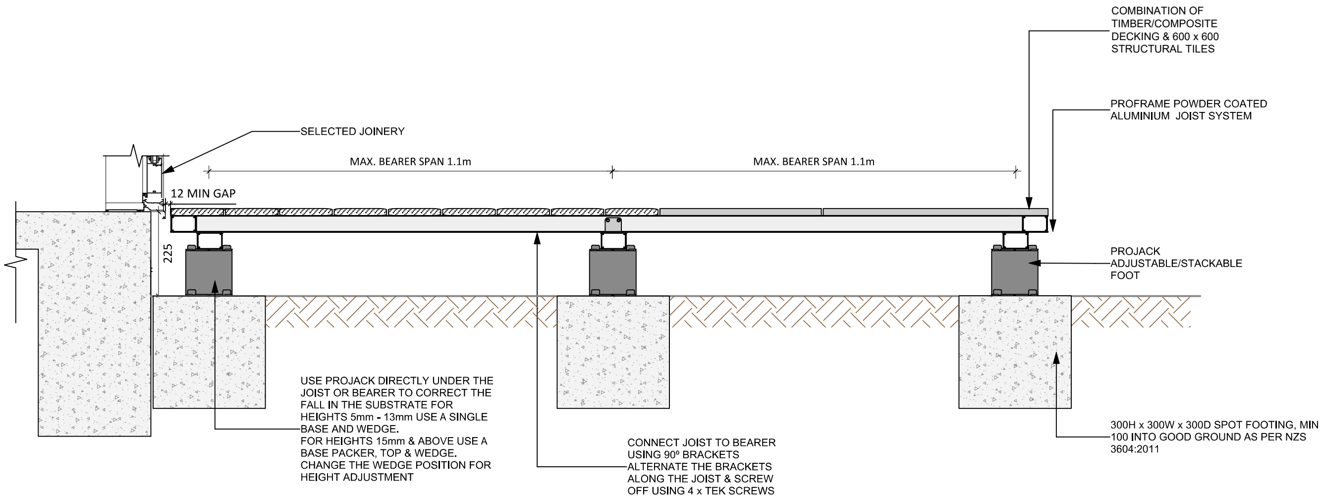
CROSS SECTION SPOT FOOTINGS ON SOIL
