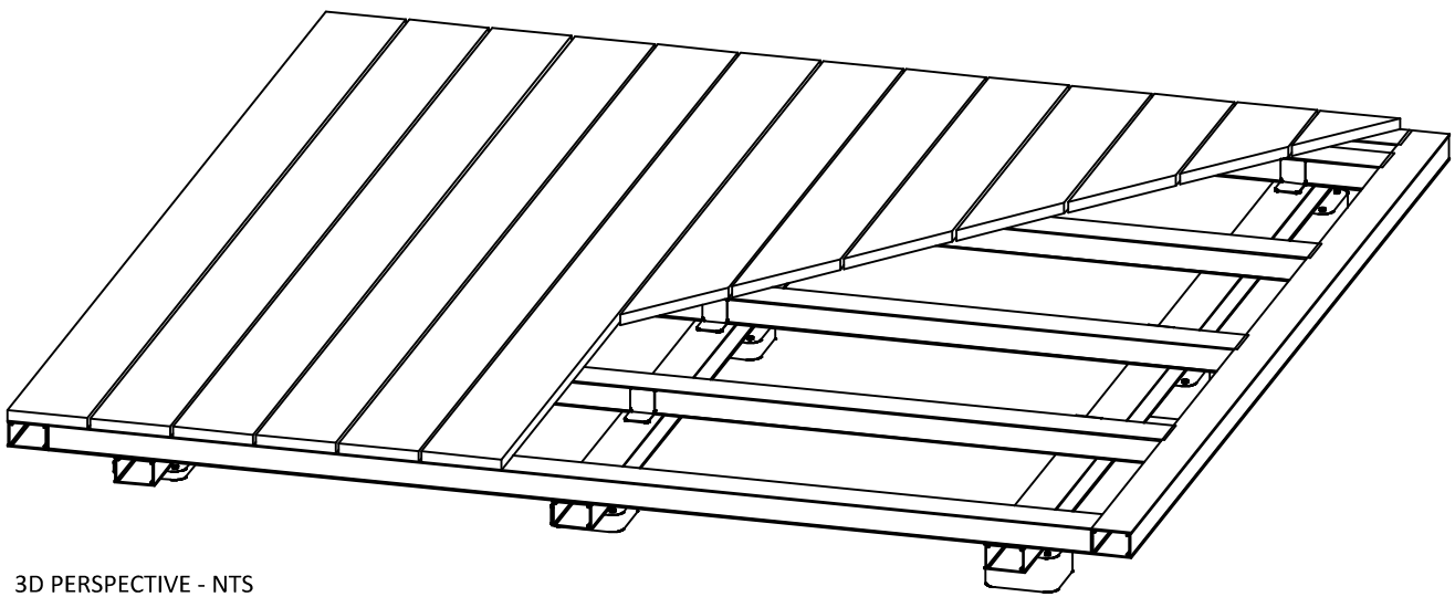
3D PERSPECTIVE - NTS
